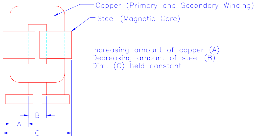
Figure 1. Basic Internal Construction
